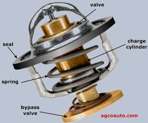
typical thermostat parts
