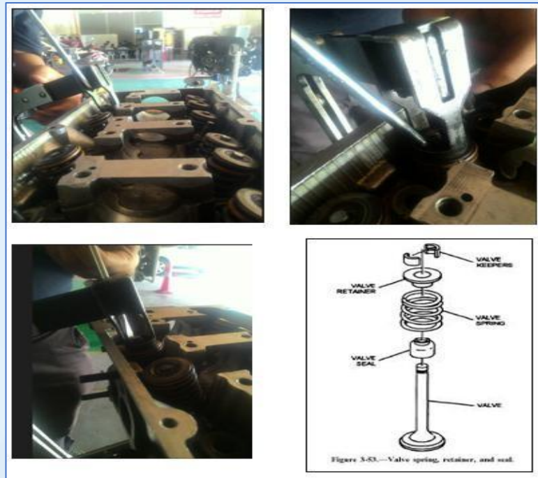
Rajah 1: Kaedah konvensional memasang valve keeper
