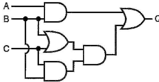
Figure 4(a)i : Logic Circuit A
