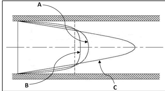
Diagram 4(a) : Velocity Profile
