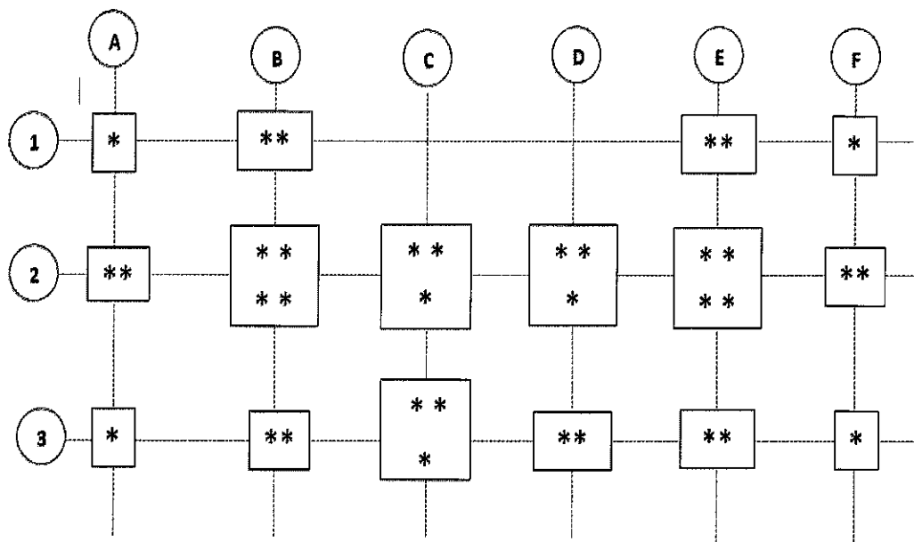
Figure B3(c) : Layout plan of piling / Rajah B3(c) : Pelan susun atur cerucuk
