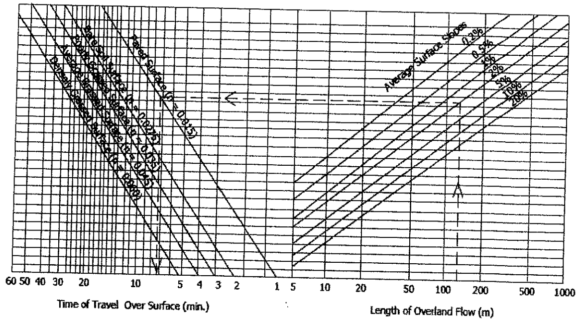
Design Chart 14.1 Nomograph for Estimating Overland Sheet Flow Times (Source: AR&R, 1977) (Overland Sheet Flow Times - Shallow Sheet Flow Only)
