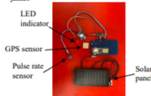
Figure 1. Complete VPFD module
