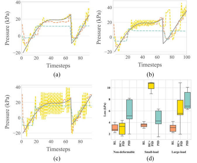
Fig. 11. Comparison with other controllers. Orange represents the RL-based controller (ours), yellow represents the handcrafted PID controller (HC+PID), and cyan represents the PID controller (PID). Gray lines are randomly referenced. (a) Controlling the pressure of nondeformable soft actuators. (b) Controlling the pressure of small soft actuators. (c) Controlling the pressure of large actuators. (d) Mean and standard deviation of seven replicates.
