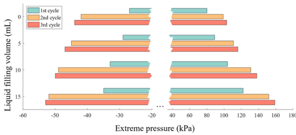
Fig. 8. Extreme pressure versus infilling liquid volume. The pump chambers were filled with water of 0, 5, 10, and 15 mL. Then, the pump executed the predefined pumping cycles three times.
