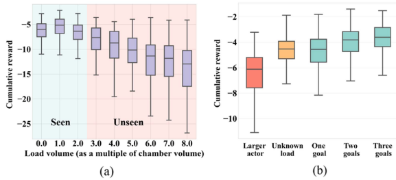
Fig. 10. Generalization and ablation study. (a) Reinforcement-learning-based pressure control generalization on seen and unseen loads in simulation. The agent was trained over small loads and being tested over small and large loads. (b) Ablation study showed that the proposed learning method (“Three goals”) achieved the best cumulative reward.
