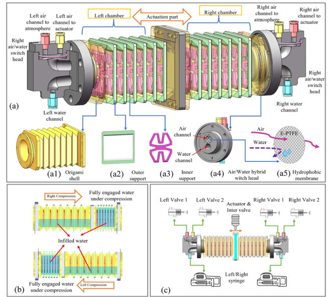
Fig. 3. Antagonistic pump designs. (a) Schematic diagram of the pump. The pump is composed of a pair of antagonistic origami chambers, chamber supports, and switch heads with hydrophobic membrane. (b) Origami chambers can expand and contract. Pneumatic pressure in the left and right chambers can be changed simultaneously by the antagonistic movement. The amount of liquid filled inside the chambers can adjust the upper and lower bounds of the pressure output range. (c) Schematic of the gas connections for the pump. The syringes are employed for liquid infilling.
