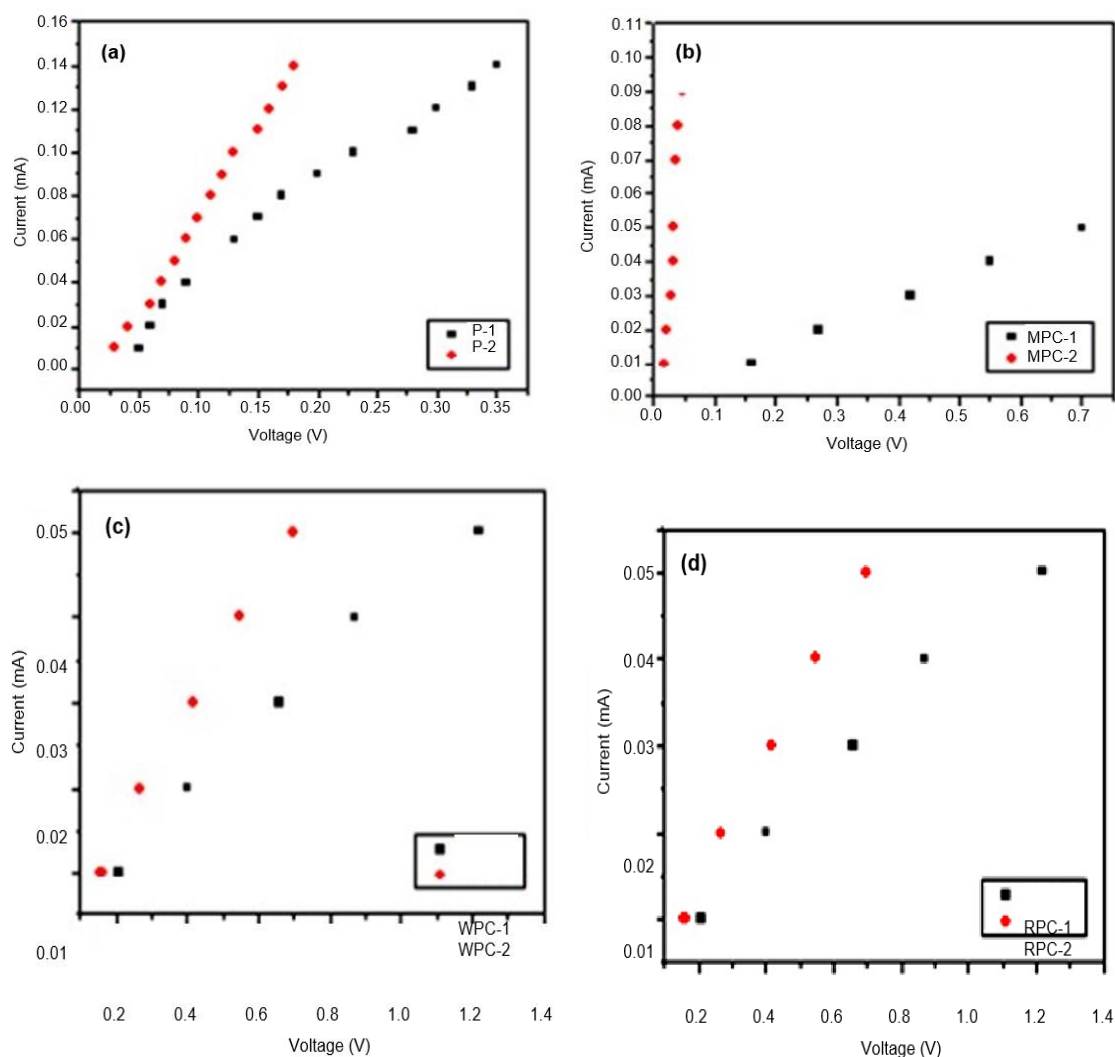
Fig. 3. Comparison of I-V characteristic curves for (a) HCl-doped polyaniline, (b) maize flour polyaniline composites, (c) wheat flour polyaniline composites at 0 and -5 °C and (d) rice flour polyaniline composites at 0 and -5 °C
