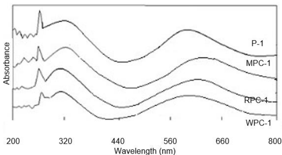
Fig. 2. (a) UV-visible spectra of polyaniline and its composites at 0 °C
