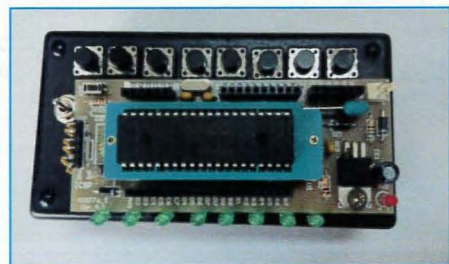
Testing Board PIC16F887
