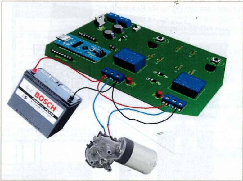
Reversible DC Motor
