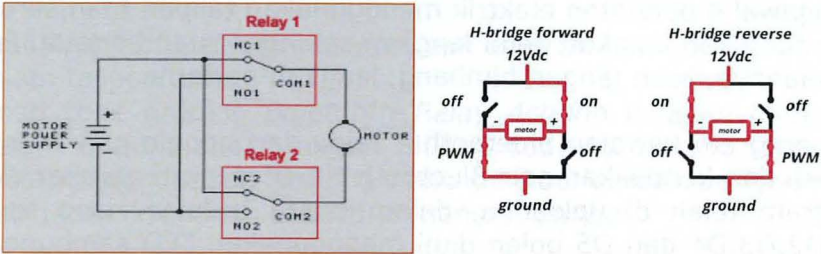
Reversible DC Motor Using 2 SPDT Relays
